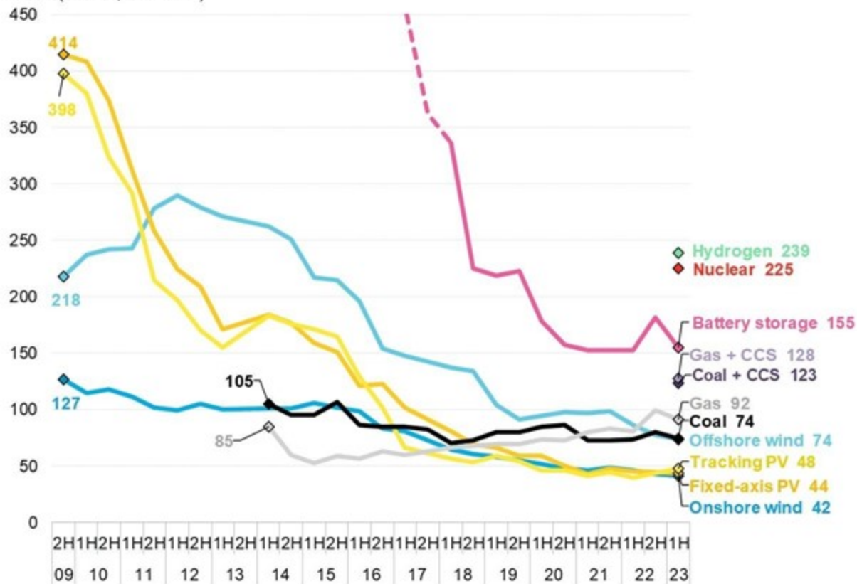
LCOE ($/MWh, real 2022)
